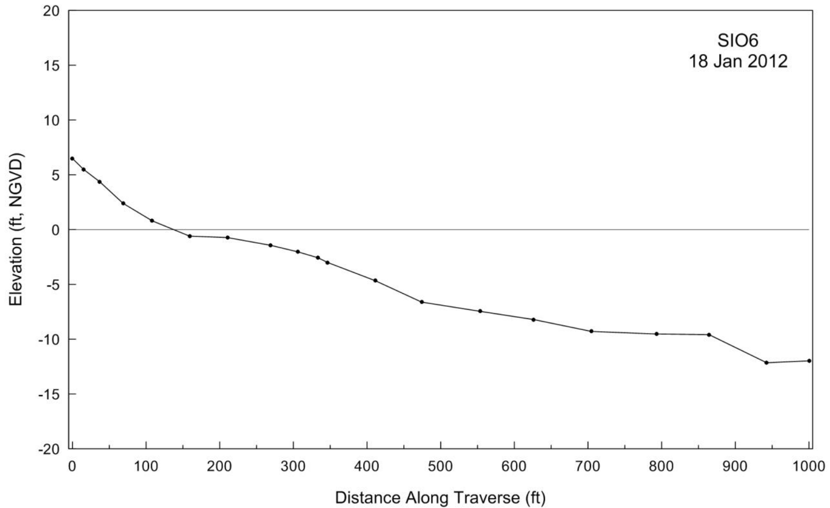
Figure A-4. Beach profile for SIO6 taken on 18 January 2012.
