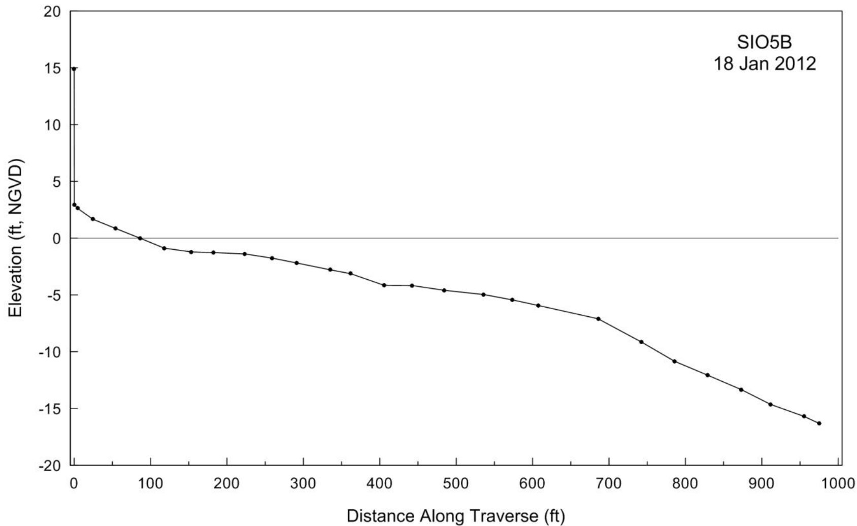
Figure A-3. Beach profile for SIO5B taken on 18 January 2012.
