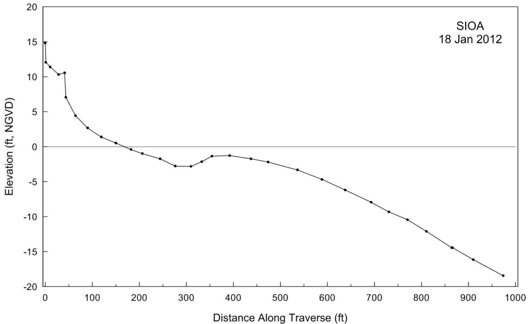
Figure A-5. Beach profile for SIOA taken on 18 January 2012.
