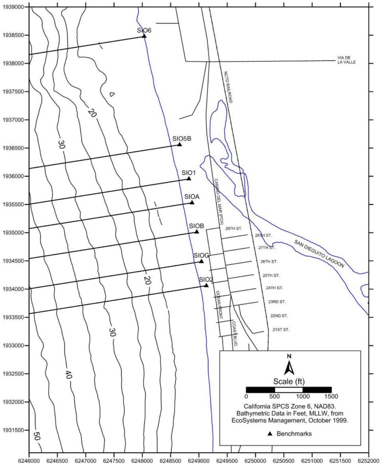
Figure 2. Beach profiles surveyed on 18 January 2012.
