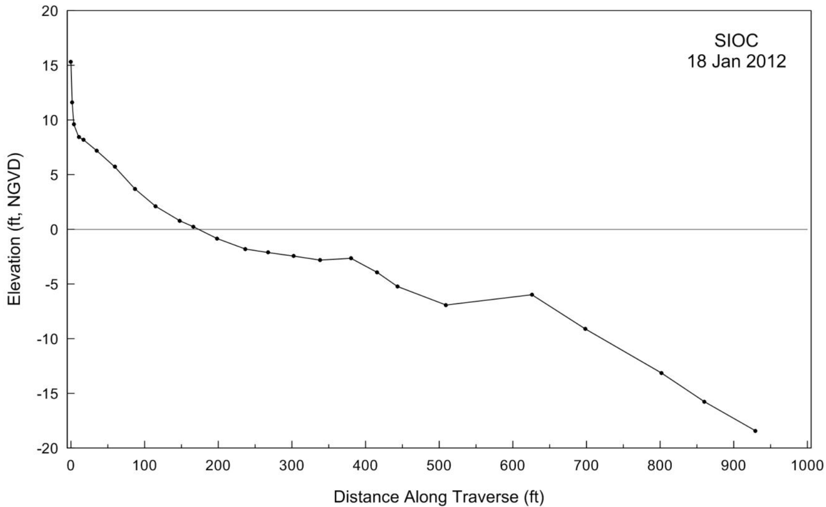
Figure A-7. Beach profile for SIOC taken on 18 January 2012.
