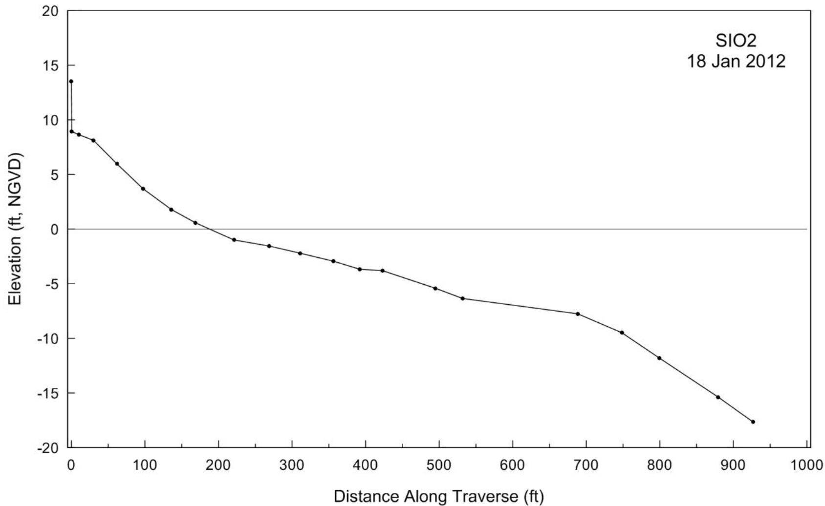
Figure A-2. Beach profile for SIO2 taken on 18 January 2012.
