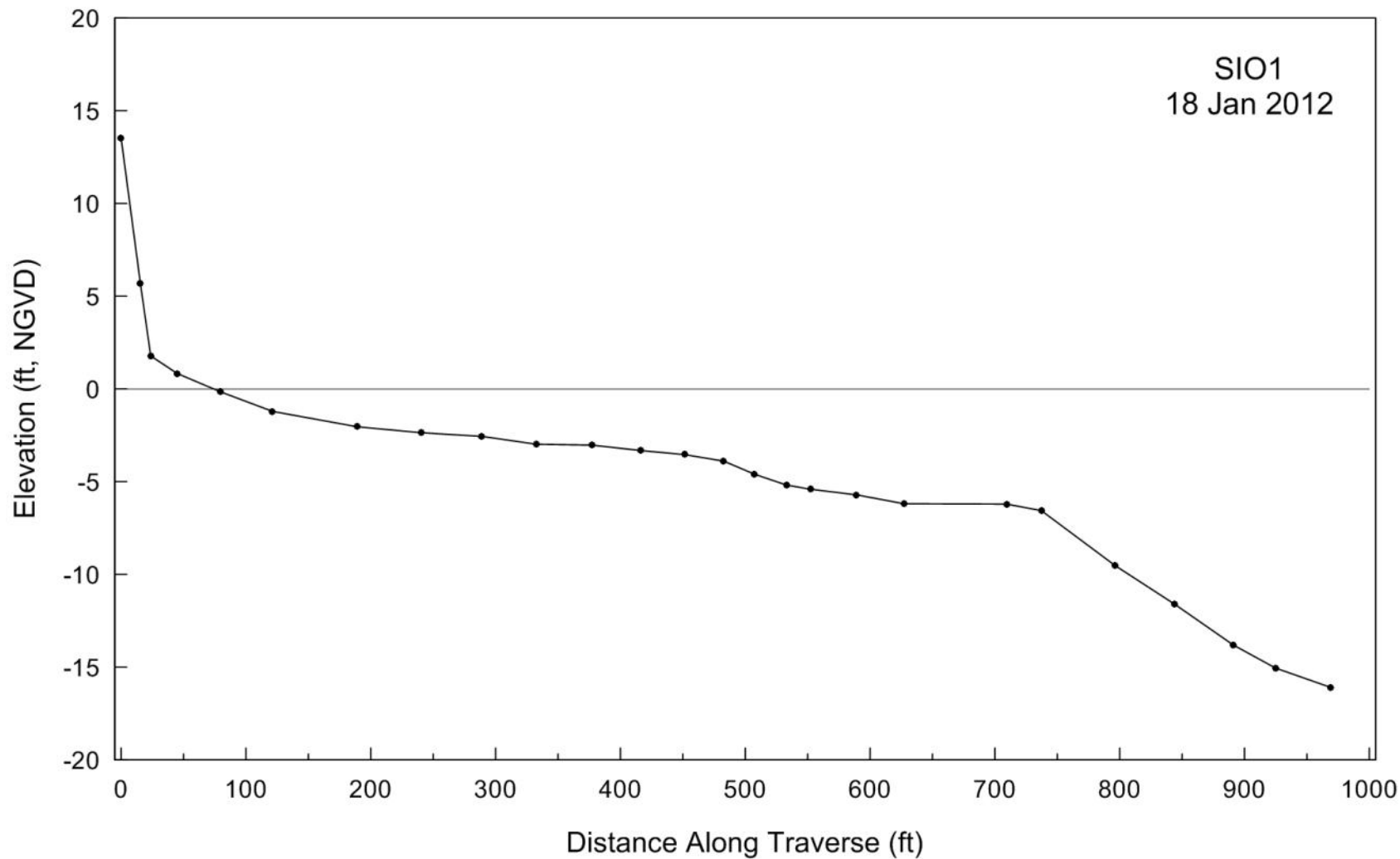
Figure A-1. Beach profile for SIO1 taken on 18 January 2012.
