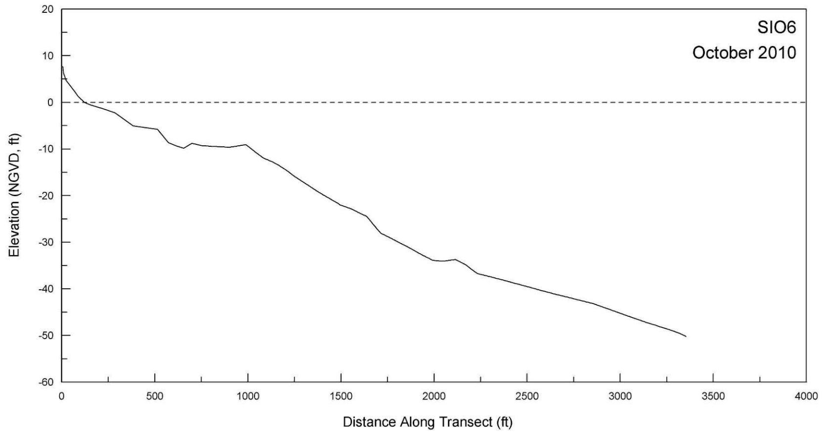
Figure A-4. Beach profile for SIO6 taken 18 October 2010.
