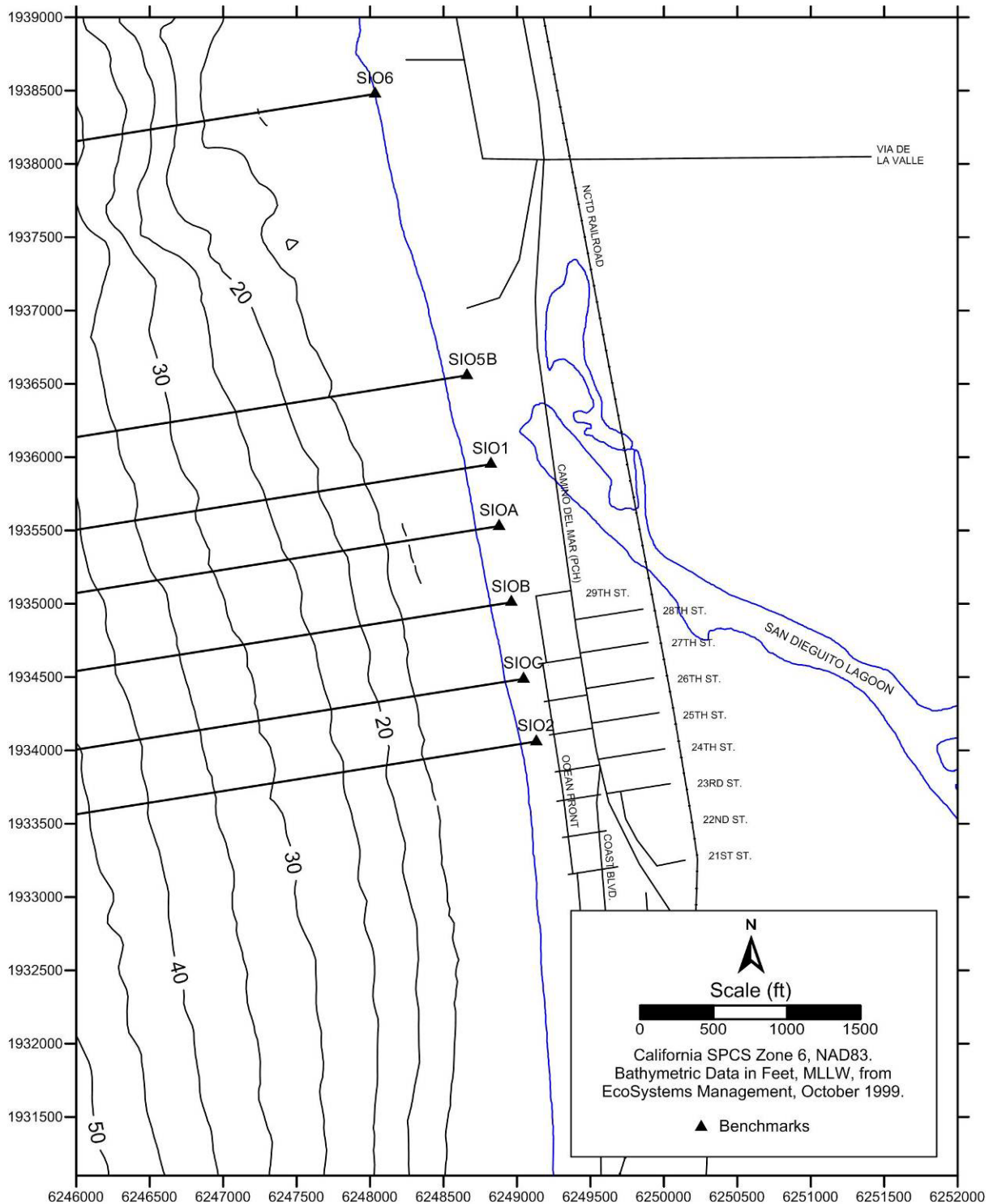
Figure 2. Beach profiles surveyed on 18 October 2010.
