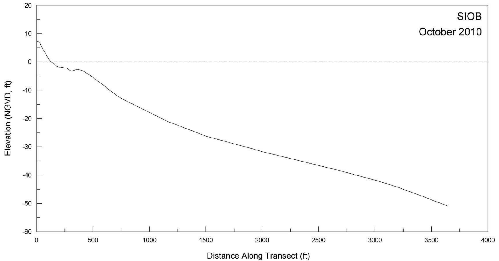
Figure A-6. Beach profile for SIOB taken 18 October 2010.
