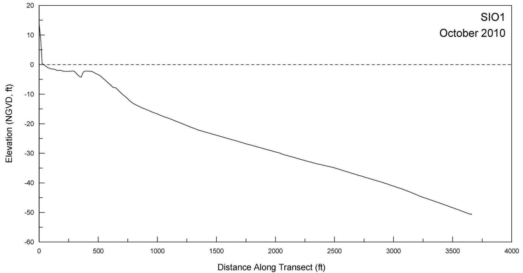
Figure A-1. Beach profile for SIO1 taken 18 October 2010.
