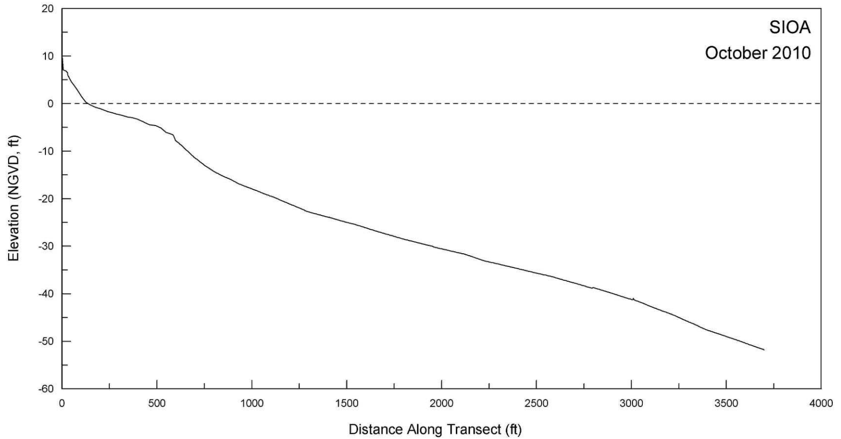
Figure A-5. Beach profile for SIOA taken 18 October 2010.
