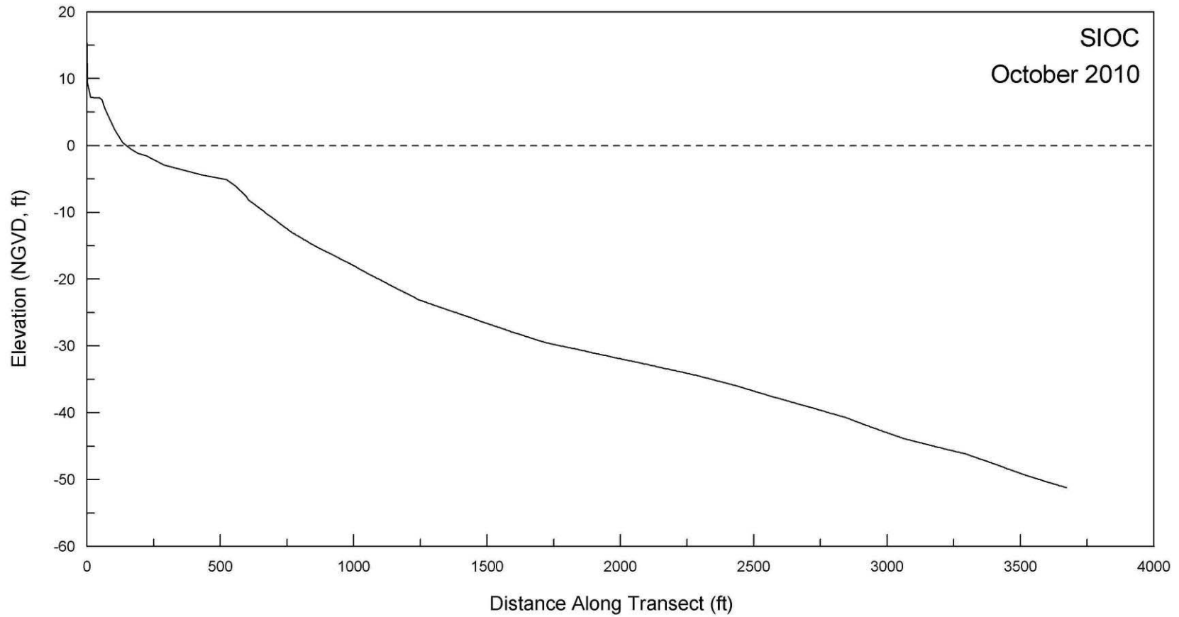
Figure A-7. Beach profile for SIOC taken 18 October 2010.
